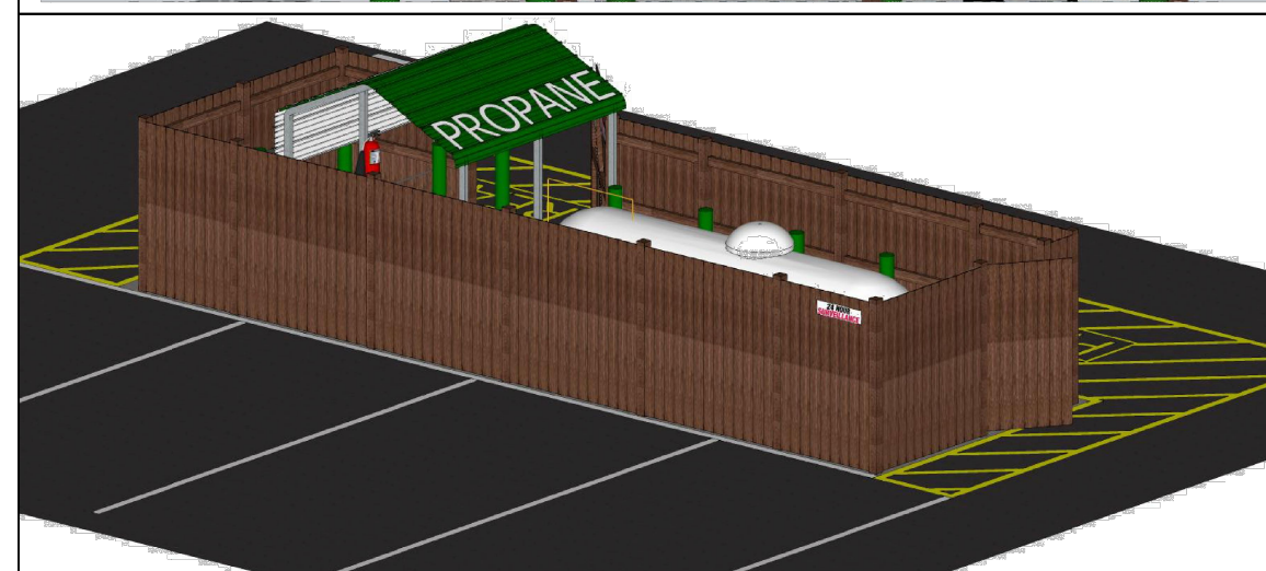
3 PROPANE FILL STATION RENDERINGS SCALE: NOT TO SCALE
