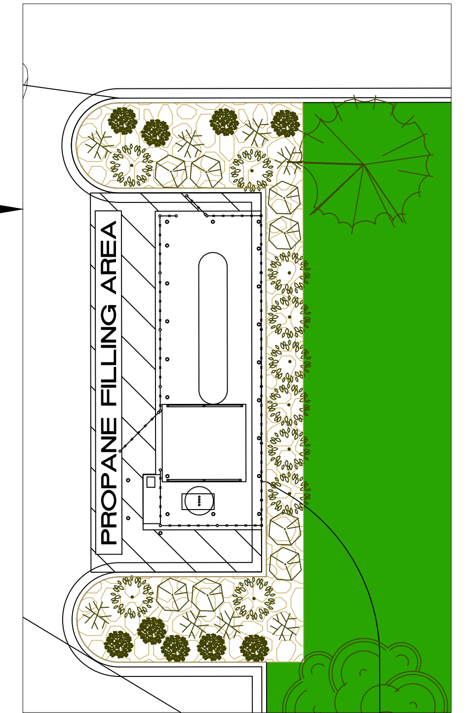
2 PROPANE FILL STATION AREA LANDSCAPING SCALE: 1" = 10'-0"
